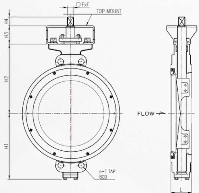
850 Series Rev B | Class 150 Wafer (Units in Inches)
