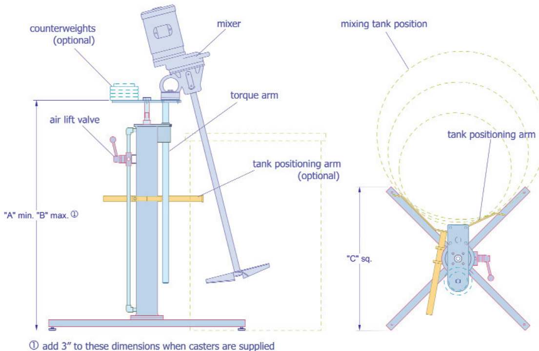
Optional casters include high-quality locking wheels and swivels.
