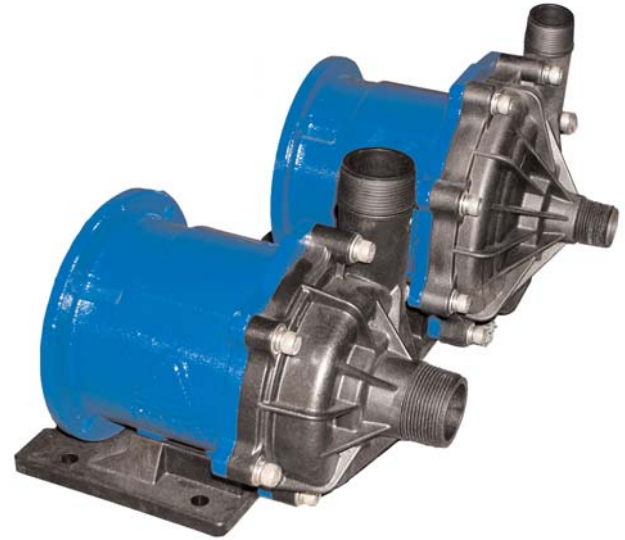
Volute casing divided into two sections
