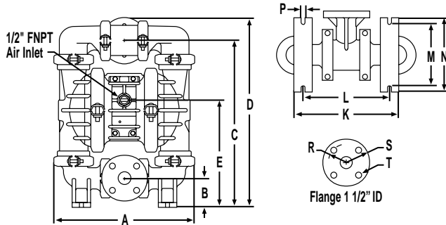
DIMENSIONS - P4 PLASTIC ITEM STANDARD (inch) METRIC (mm)
