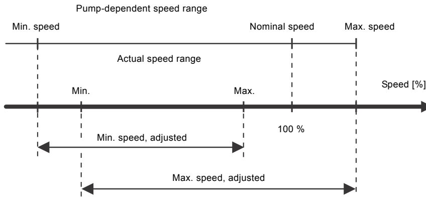
Fig. 29 Setting of the min. and max. curves in % of maximum performance
