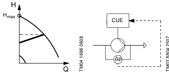
Fig. 33 Proportional differential pressure, H_{max} update
