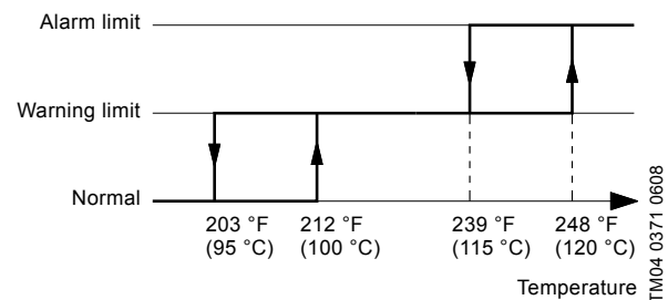
Fig. 30 Monitoring of bearing temperature with warning and alarm limits
