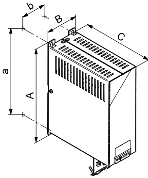
Fig. 65 Wall mounting
