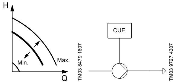
Fig. 5 Open loop, constant curve
