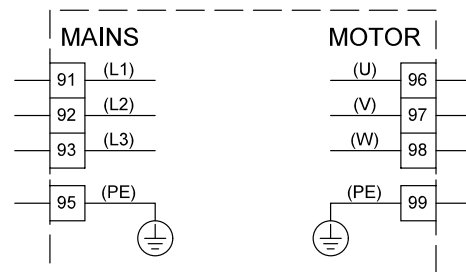
Fig. 40 Wiring diagram, three-phase power supply connection
