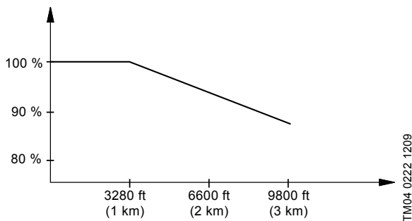
Fig. 51 Derating of output current at low air pressure
