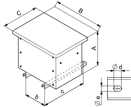
Fig. 66 Floor mounting
