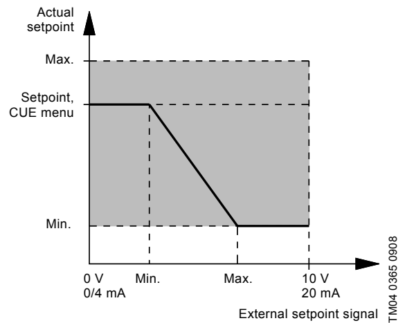
Fig. 20 Reduced inverse external setpoint signal
