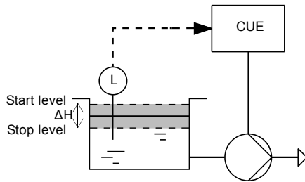
Fig. 27 Constant level with stop function. Difference between start and stop levels ( \Delta H )
