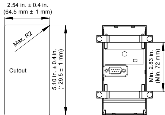
Fig. 60 Cabinet mounting, dimensions of cutout
