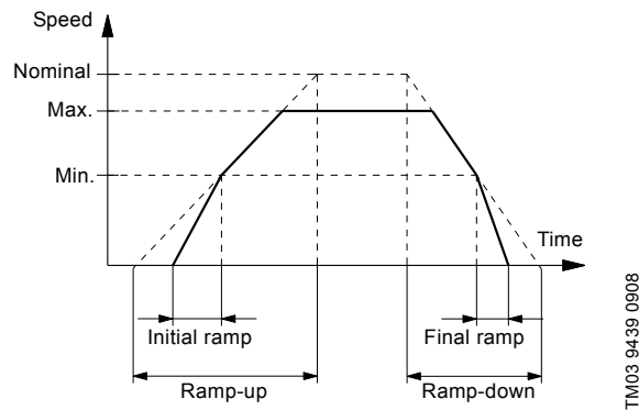
Fig. 31 Ramp-up and ramp-down of the CUE
