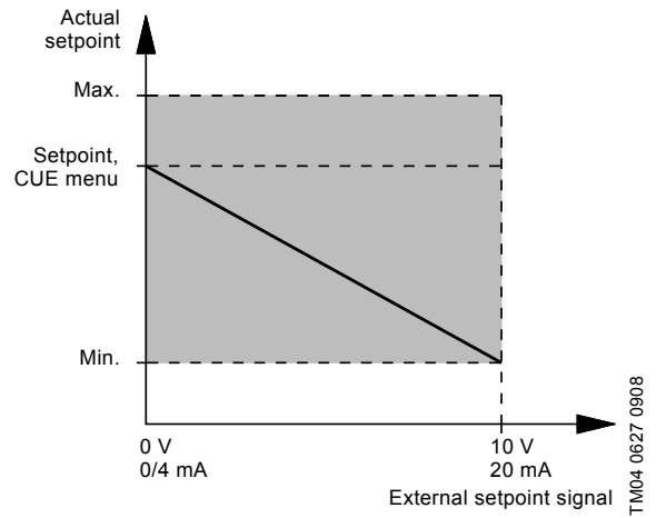
Fig. 19 Inverse external setpoint signal
