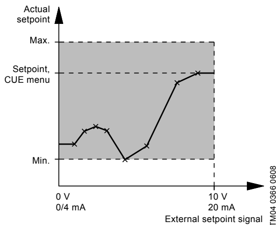
Fig. 22 External setpoint based on a reference table
