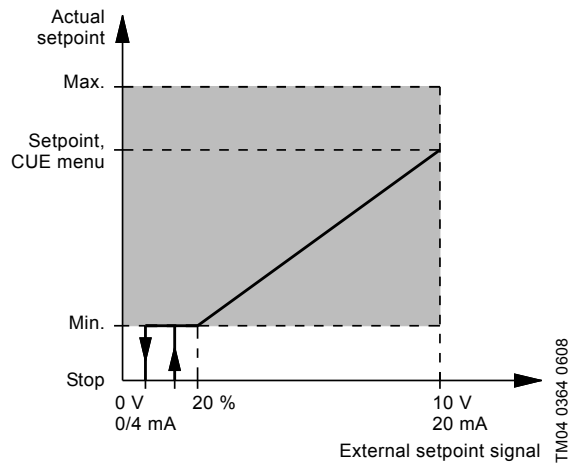
Fig. 21 External setpoint with stop function
