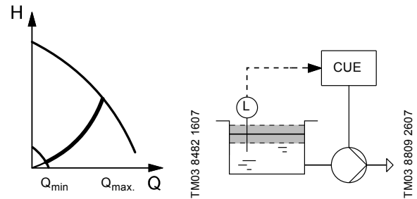
Fig. 12 Constant level with stop function
