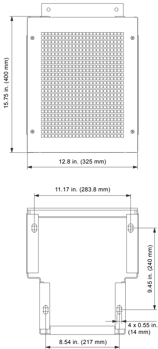
Fig. 61 Drilling template for pedestal [in. (mm)]
