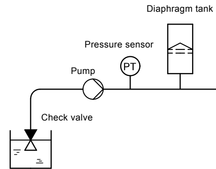
Fig. 25 Position of the check valve and pressure sensor in a system with suction lift operation
