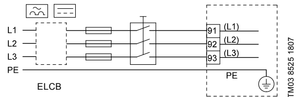
Fig. 39 Example of three-phase power supply connection of the CUE with power supply switch, backup fuses and additional protection
