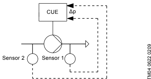
Fig. 34 Differential pressure from two sensors
