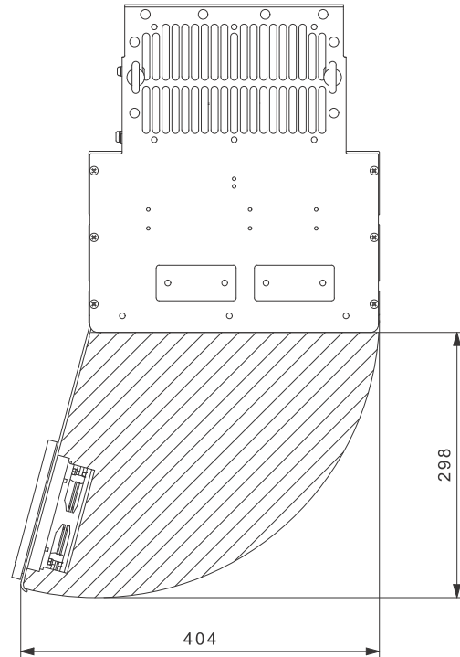
Fig. 38 Free space in front of CUE enclosures D1h and D2h
