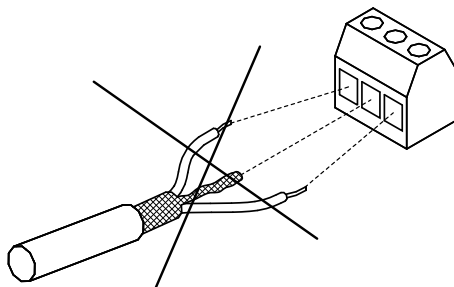
Fig. 46 Do not twist the screen ends.
