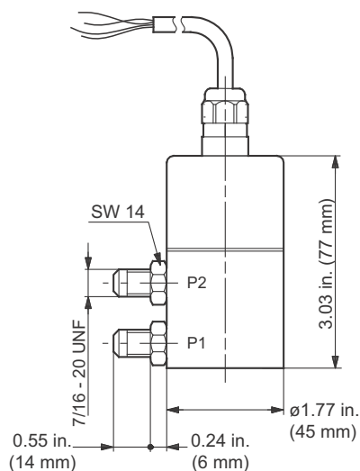
Fig. 68 Dimensions, DPI
