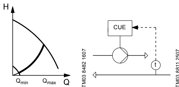
Fig. 14 Constant temperature
