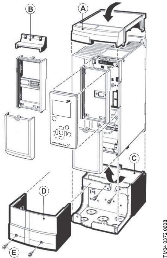
Fig. 63 Example of IP21/NEMA1 option for enclosure A3
