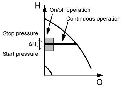
Fig. 24 Constant pressure with stop function. Difference between start and stop pressures ( \Delta H )
