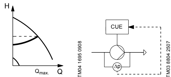
Fig. 32 Proportional differential pressure, parabolic curve
