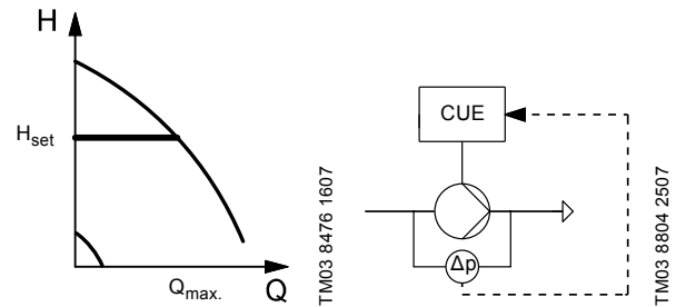
Fig. 7 Constant differential pressure, pump
