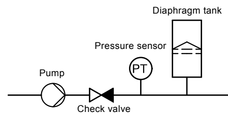
Fig. 26 Position of the check valve and pressure sensor in a system with positive inlet pressure
